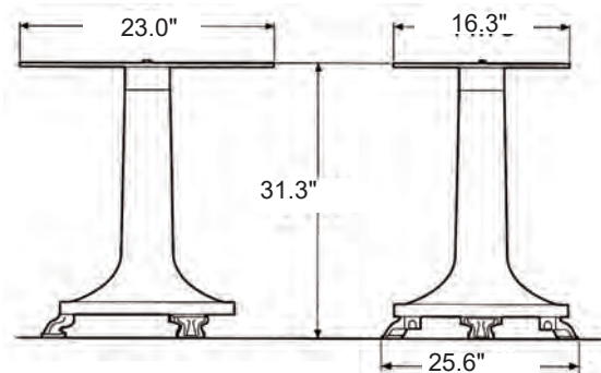
330V-130-STAND (sold separately)
