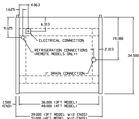
3' & 4' Plan Views
