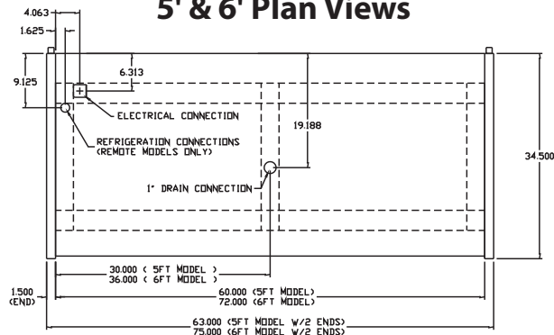
5' & 6' Plan Views
